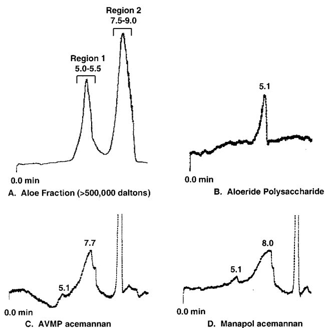
Figure 2. Size-exclusion HPLC chromatograms: (a) aloe vera juice high-molecular-weight fraction (>500 000 molecular weight cutoff), 75 \mu\text{L} injection at 10 mg/mL; (b) purified Aloeride polysaccharide, 20 \mu\text{L} injection at 1.8 mg/mL; (c) AVMP acemannan preparation, 100 \mu\text{L} injection at 1 mg/mL; (d) Manapol acemannan preparation, 100 \mu\text{L} injection at 1 mg/mL.
